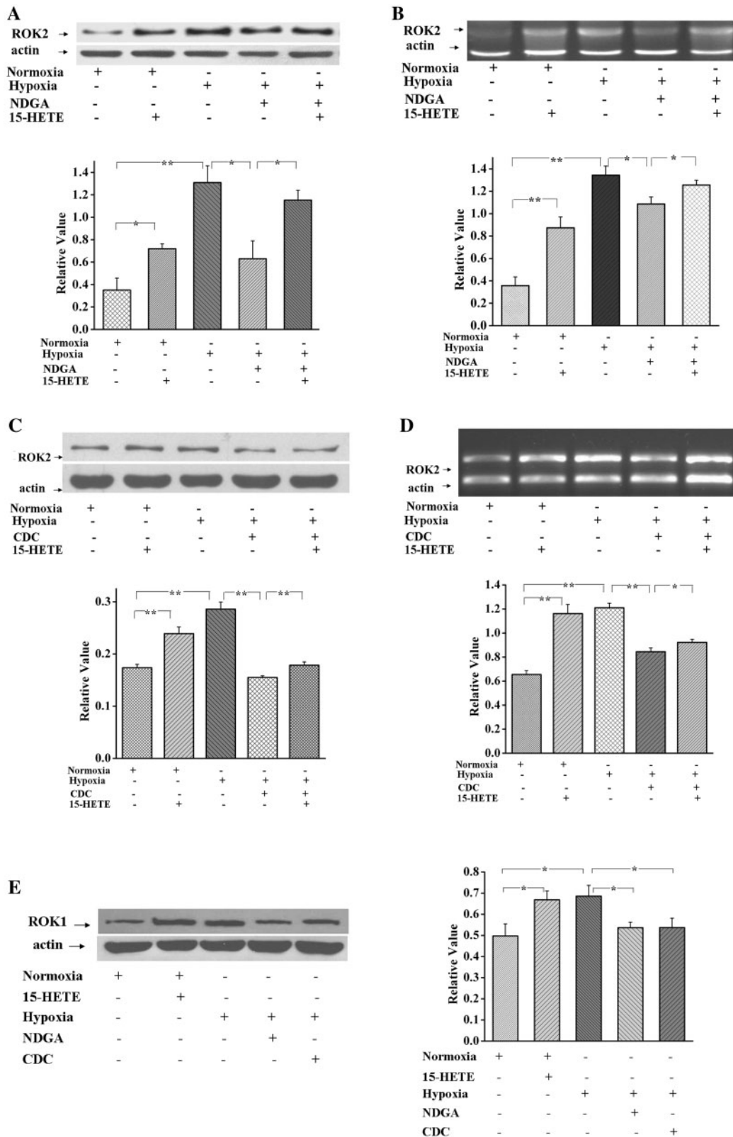
Fig. 4 Effects of 15-HETE on the expression of ROK in cultured PSMCs. The experimental groups were as follows: group 1 was normoxic control; group 2 was 15-HETE group, in which the cells were treated with 1 \mu M 15-HETE for 24 h under normoxic condition; group 3 was hypoxic group in which the cells were treated under hypoxic condition for 24 h; group 4 was subjected to inhibition of endogenous 15-HETE, in which the cells were pretreated with 30 \mu M NDGA or 5 \mu M CDC for 24 h under hypoxic condition; group 5 was exposed to exogenous 15-HETE and hypoxia, in which the cells were treated with 1 \mu M 15-HETE under hypoxic condition after blocks of endogenous 15-HETE with NDGA or CDC for 24 h. ROK2 protein expression in PSMCs treated with NDGA (A) and CDC (C) under hypoxic condition. ROK2 mRNA expression in PSMCs treated with NDGA (B) and CDC (D) under hypoxic condition. E: represented the effect of 15-HETE on the expression of ROK1 protein. All values are denoted as mean \pm SEM ( n = 3 , * P < 0.05 , ** P < 0.01 ).
